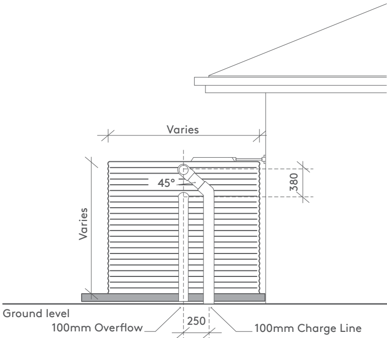
SIDE ELEVATION TYPICAL
