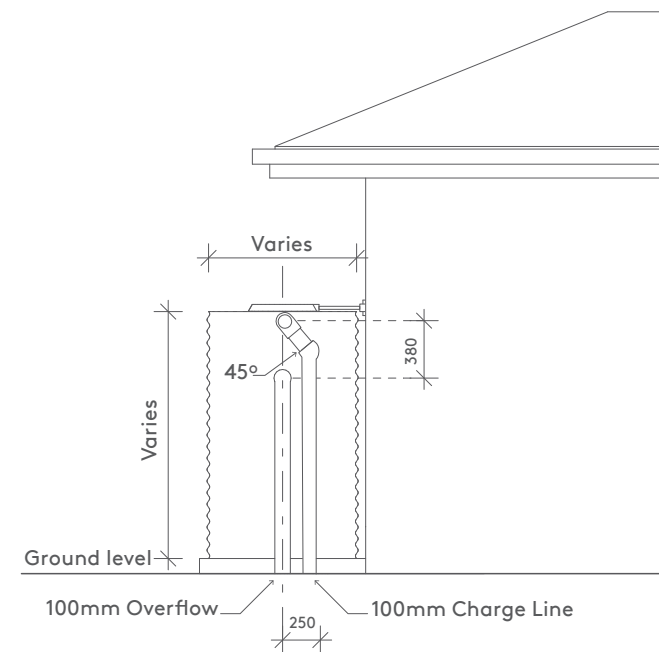
SIDE ELEVATION TYPICAL
