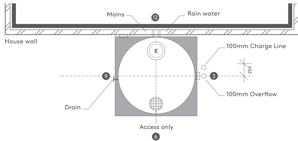
PLAN VIEW TYPICAL
