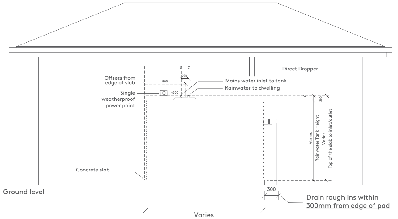
FRONT ELEVATION OPTION A
