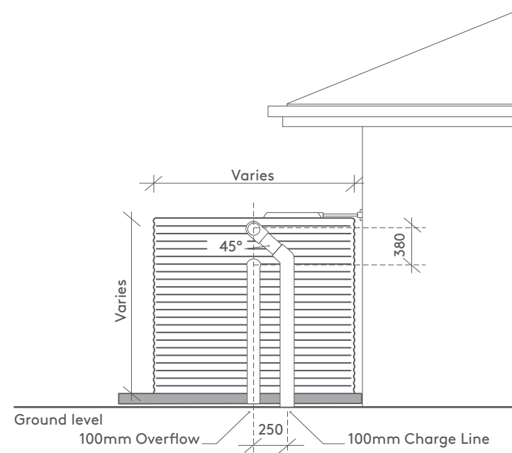
SIDE ELEVATION TYPICAL
