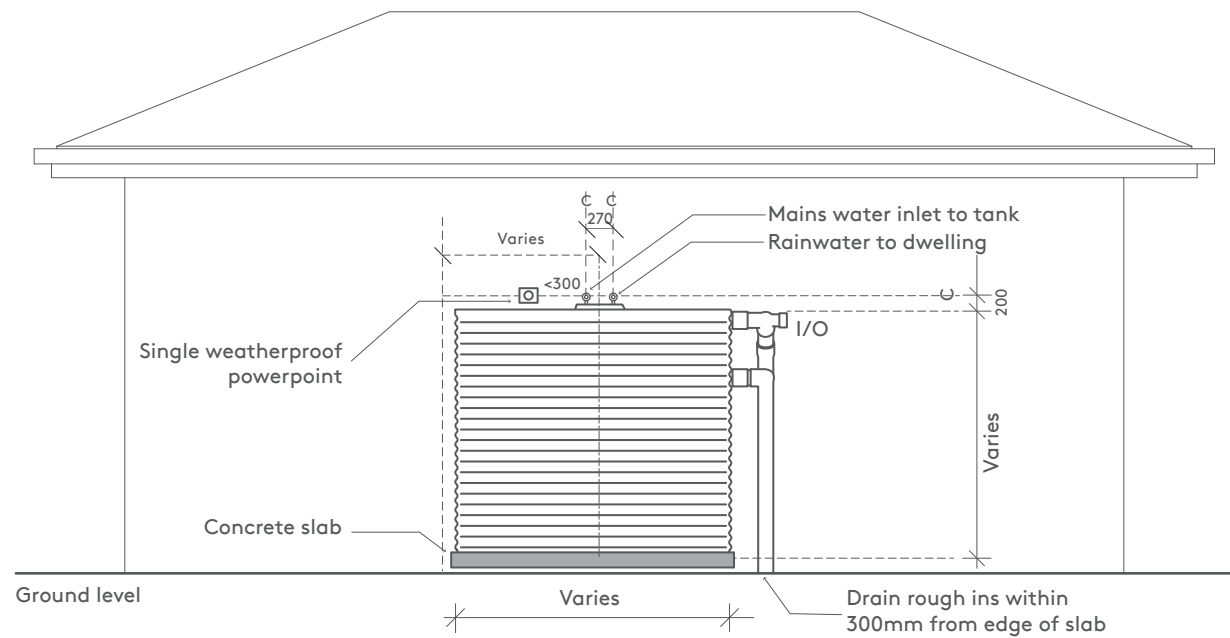
FRONT ELEVATION OPTION A
