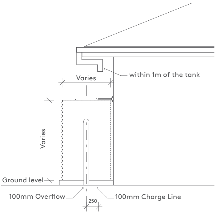
SIDE ELEVATION TYPICAL
